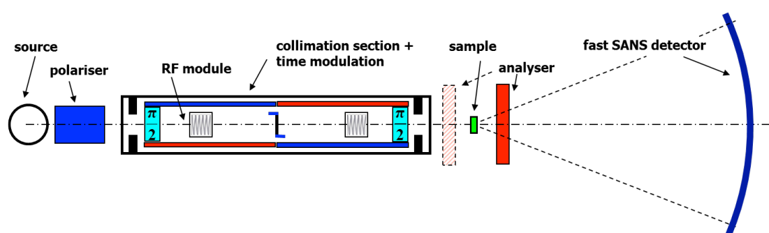
Fig.3: Schematic diagram in side view of the proposed pin-hole SANS instrument in combination with MIEZE. The two RF modules are tuned in such a manner that the intensity at the SANS detector has a fast modulation in time.
