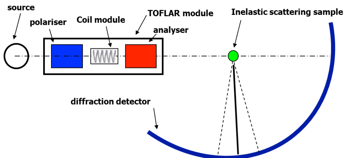
Fig. 6: Schematic drawing (not in scale) of a TOFLAR module introduced at the incoming beam of a powder diffractometer. The module consists of a precession field between a polariser creates an intensity modulation as a function of wavelength and magnetic field. Due to inelastic scattering the amplitude of this modulation will decrease.
