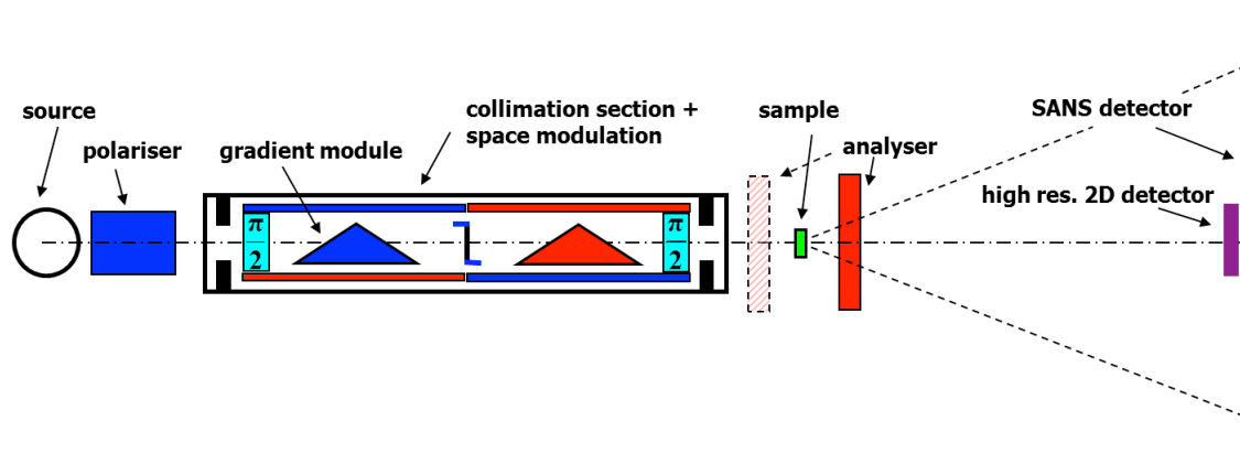
Fig.2: Schematic diagram in side view of the proposed pin-hole SANS instrument in combination with modulated SESANS. The \pi/2 -flippers mark the start and end of the precessions and between the precession elements there is a field stepper. A high-resolution position sensitive detector with low efficiency is used instead of beam stop. This could be stationary and be used in all configurations.
