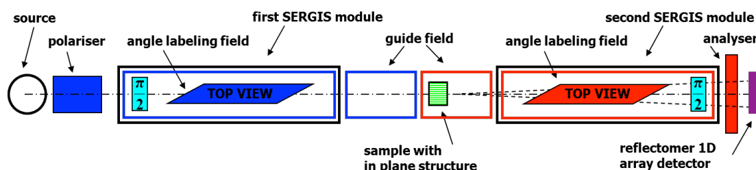
Fig.4: Schematic diagram in top view of the proposed spin-echo option for reflectometry.
