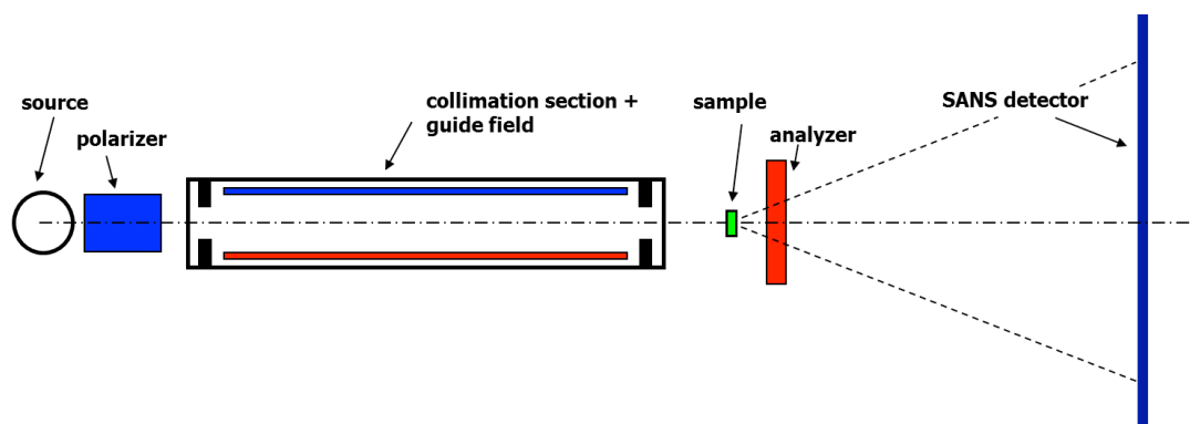
Fig.1: Schematic diagram in side view of the proposed pin-hole SANS instrument with polarized neutrons for which the add-on modules will be designed.
