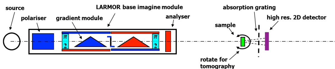
Fig. 5. Schematic view of an imaging station with a Larmor labelling add-on at the incoming beam. Two Larmor precession fields with a gradient create a modulation of the intensity at the absorption grating before the detector. Effectively, they replace the two gratings used in conventional phase contrast or dark field imaging. The sample is on a rotation stage for the tomographic reconstruction.
